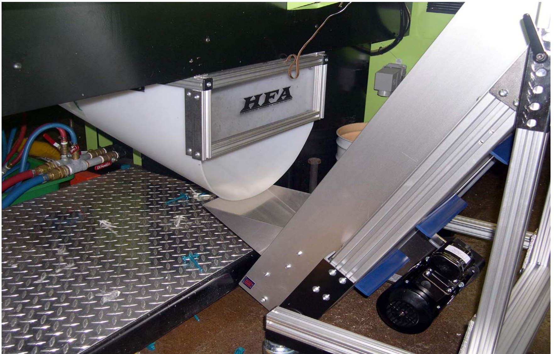
White UHMW Under Press Chute Feeding HFA 2220 Model Conveyor
