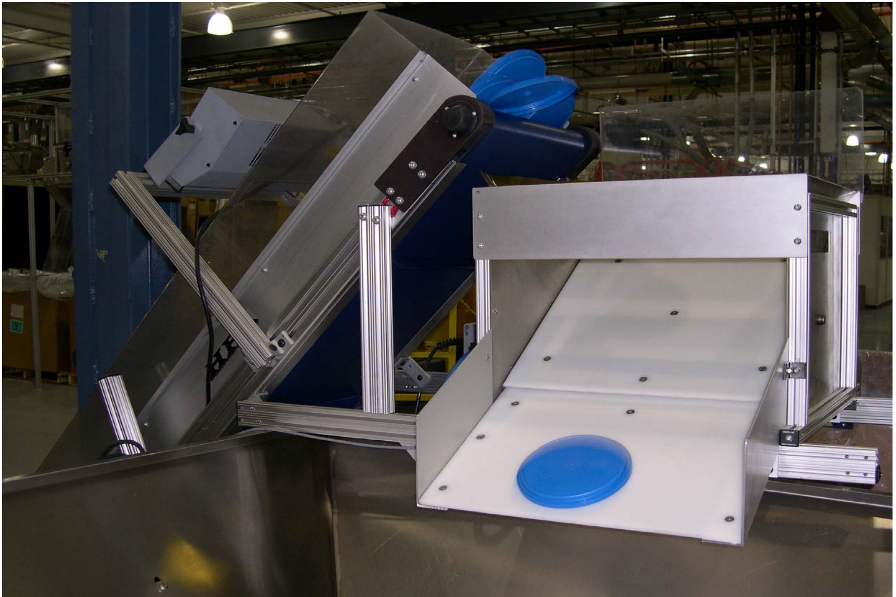
Diverter Mounted at Discharge End Feeding Parts into a Hopper
