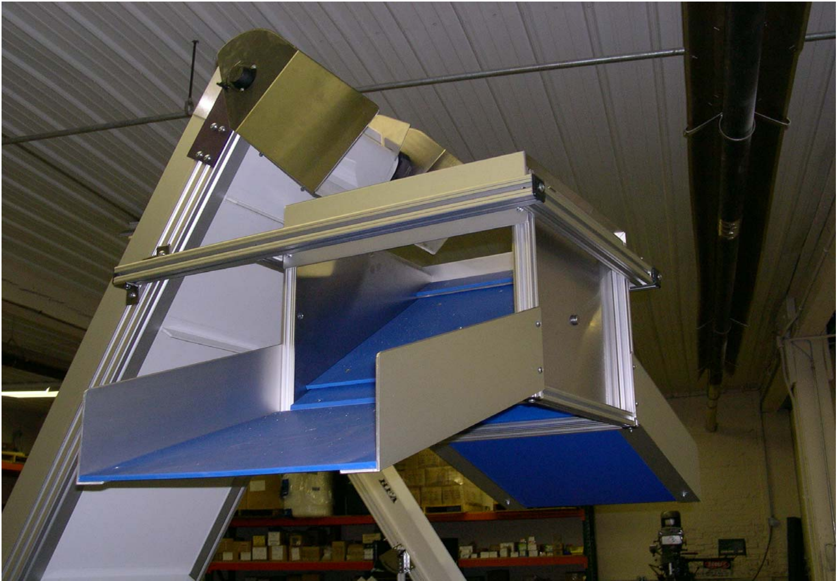
Diverter Mounted at Discharge End of HFA 2220 Series Conveyor Designed to Fill (2) Gaylords by Count or Weight
