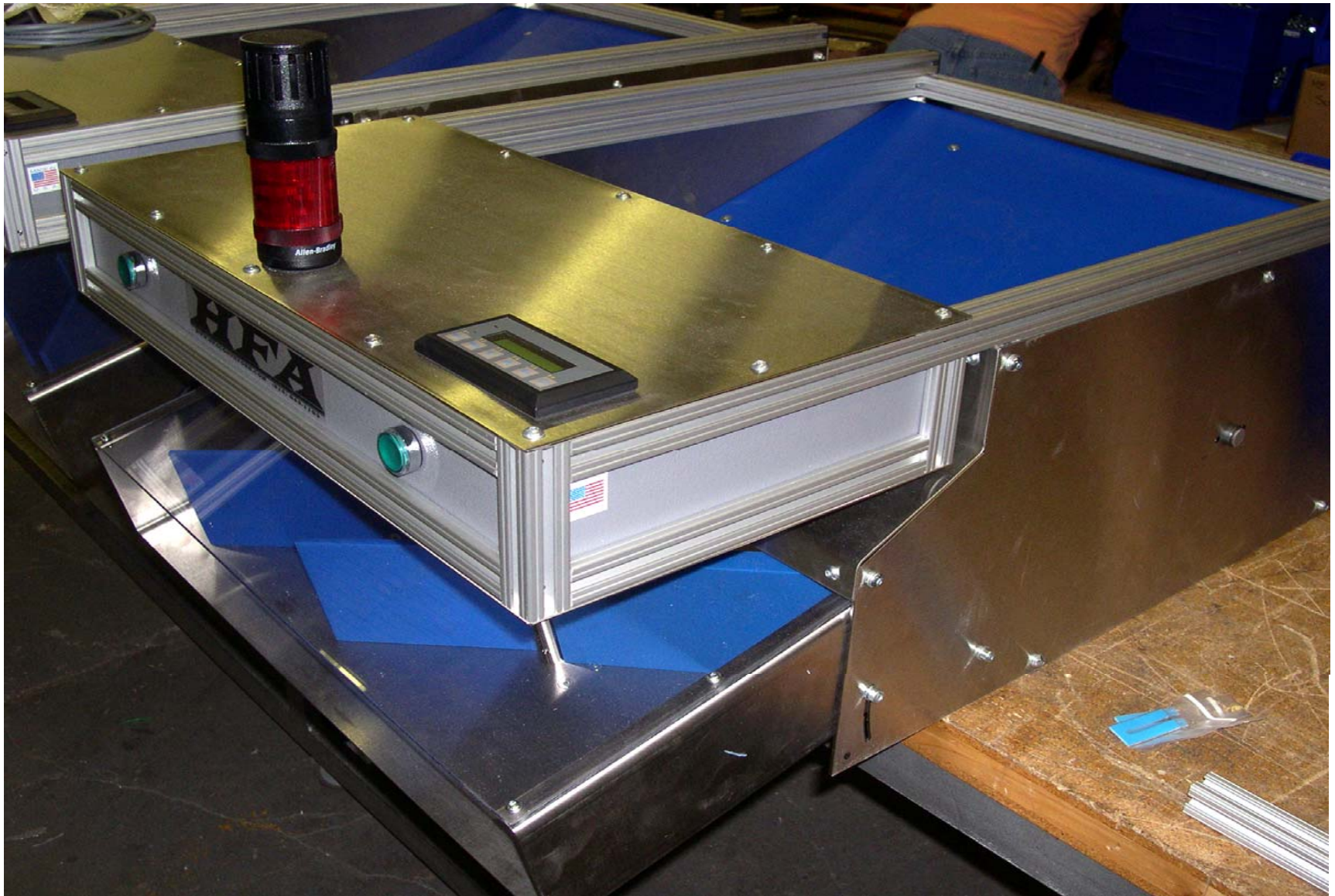
Custom Diverter Designed to Fill (2) Totes by Count From Under the Press
