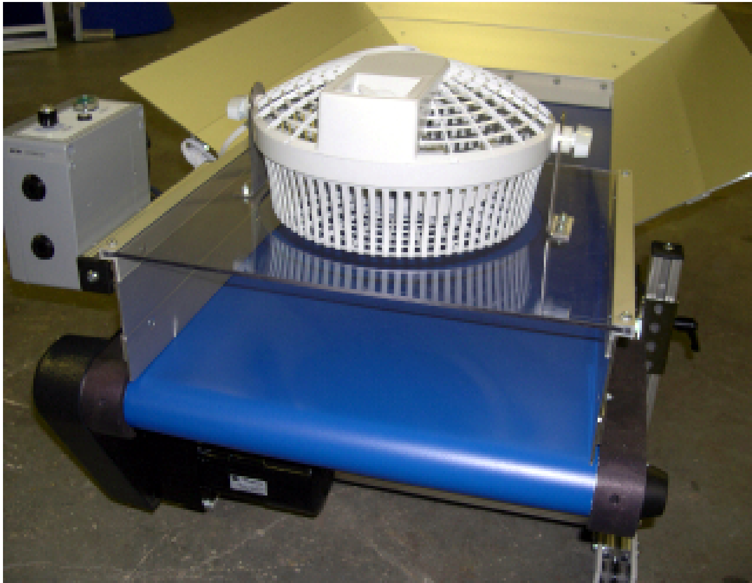
Ambient Cooling Fan with Lexan Cover on an HFA 2210 Under-Press Conveyor
