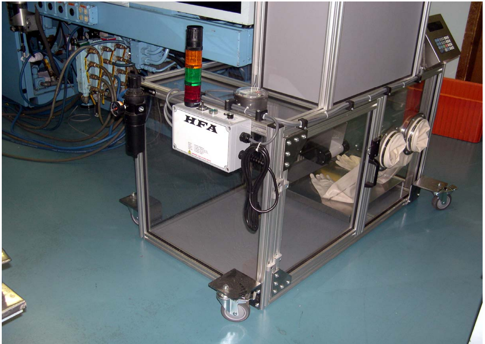
Clean-room Under Molding Machine Fed by an HFA 2210 Model Conveyor
