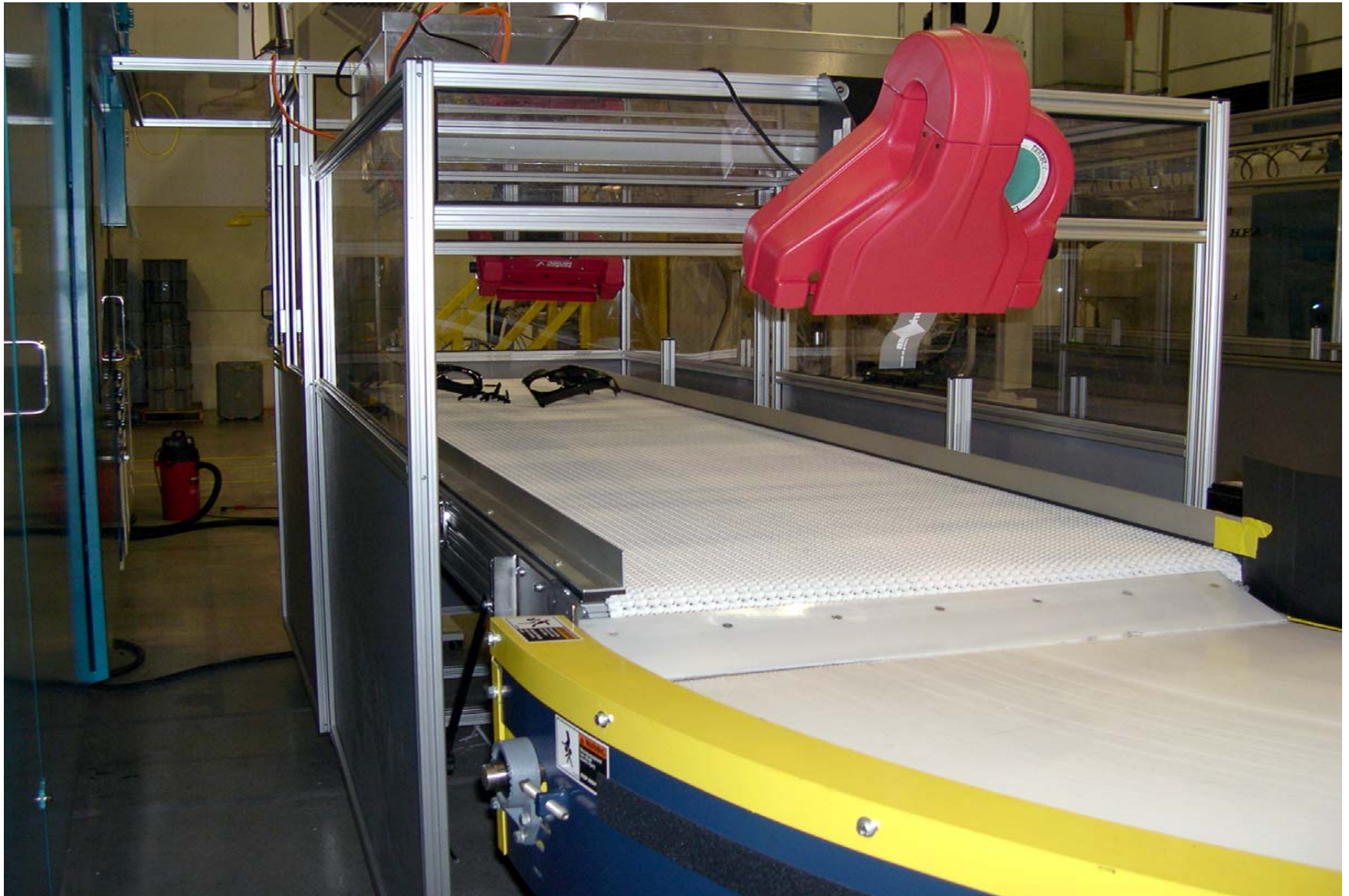
Static-Elimination Blower Mounted to an HFA 2210 Model Conveyor with Plastic Link Belting
